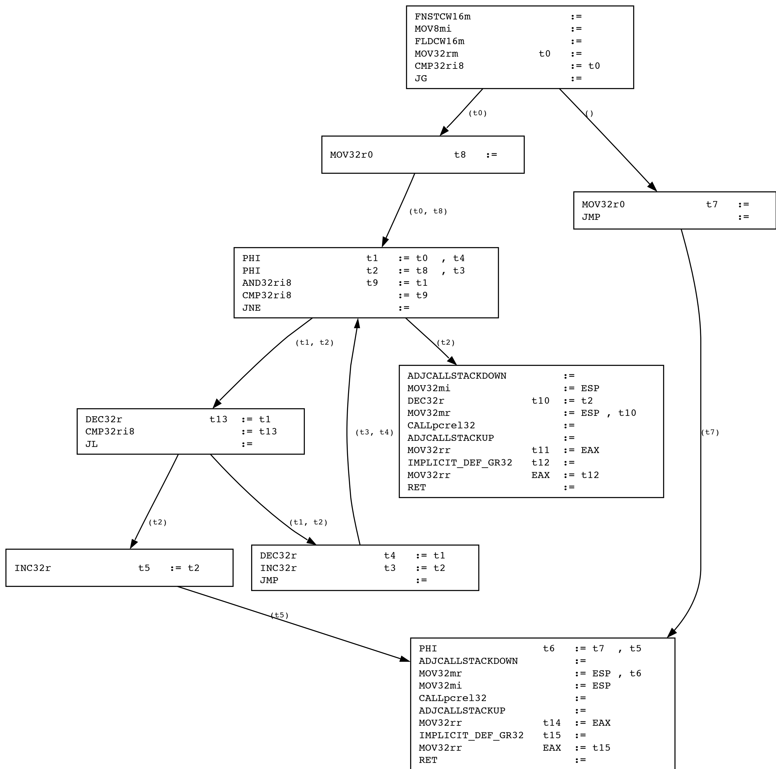
CFG for function main
